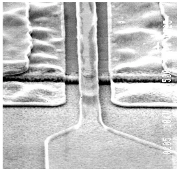
Fig.1: SEM photograph of 1 \mu\text{m} -gate AlGaN/GaN HEMT
