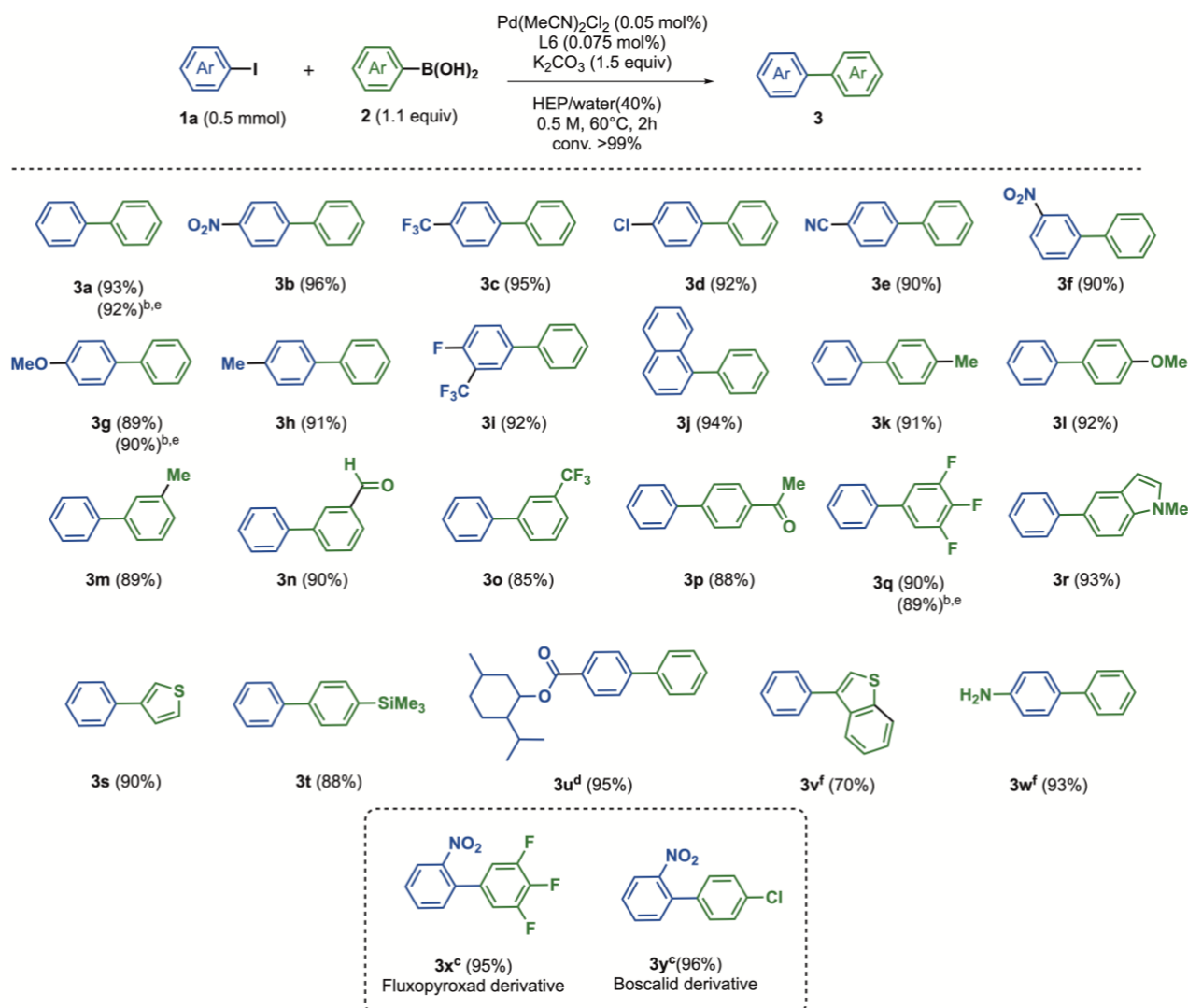
Scheme 1. Scope of aryl iodides and aryl boronic acids.
