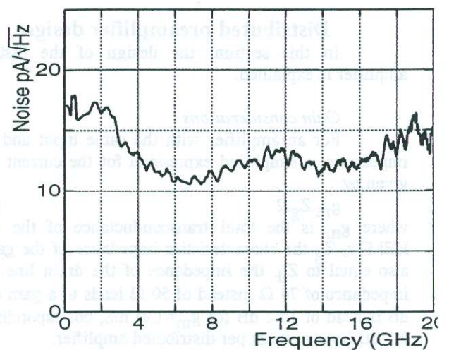
Fig 6: Equivalent input noise. The average equivalent input noise is 13 pA/√Hz over 14 GHz.
