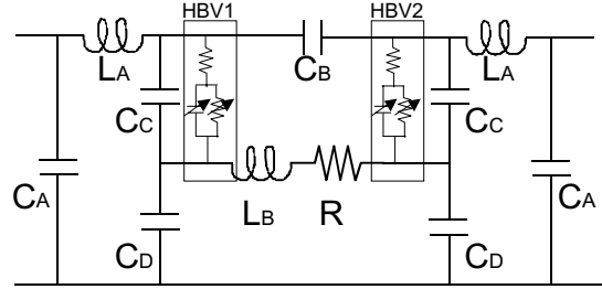
Fig. 6. Lumped element circuit considered in the case of the coplanar HBV structure; the boxed regions represent the equivalent circuit of the HBV structures.
