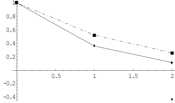
Figure 1: \underline{\delta}_t (continuous line) and \bar{\delta}_t (discontinuous line) as a function of t . D' = 2.5 , D = 2 , \phi = 1 . The star indicates \delta^* .
