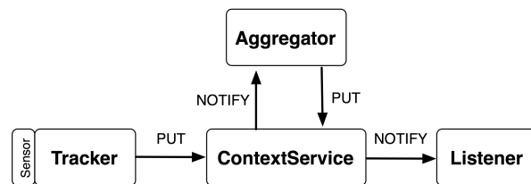
Figure 3: MobiComp infrastructure.
