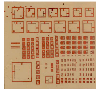
Fig. 4b. LCP test coupon
