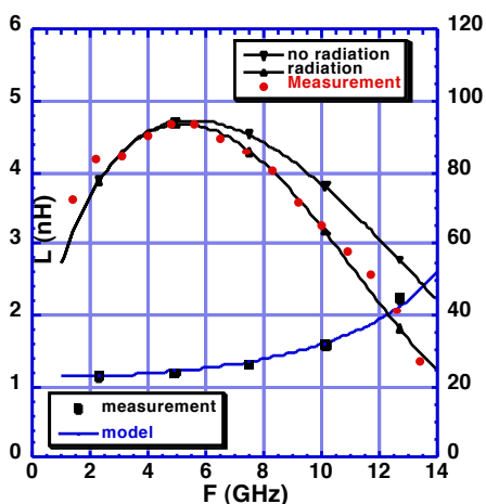
Fig. 4a. Measurement performances of High Q RF inductors.
