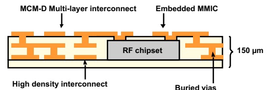
Fig. 3a. Concept view of Ultra-compact module.
