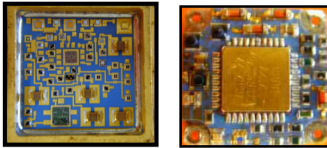
Figure 7: TCXO circuit
